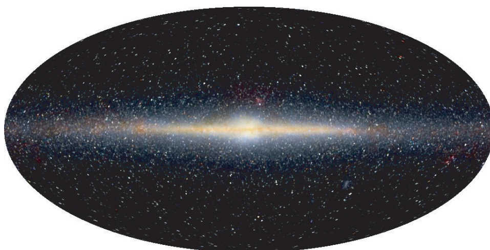
FIGURE 88 A false colour image of how the night sky, and our galaxy in particular, looks in the near infrared (courtesy NASA).
